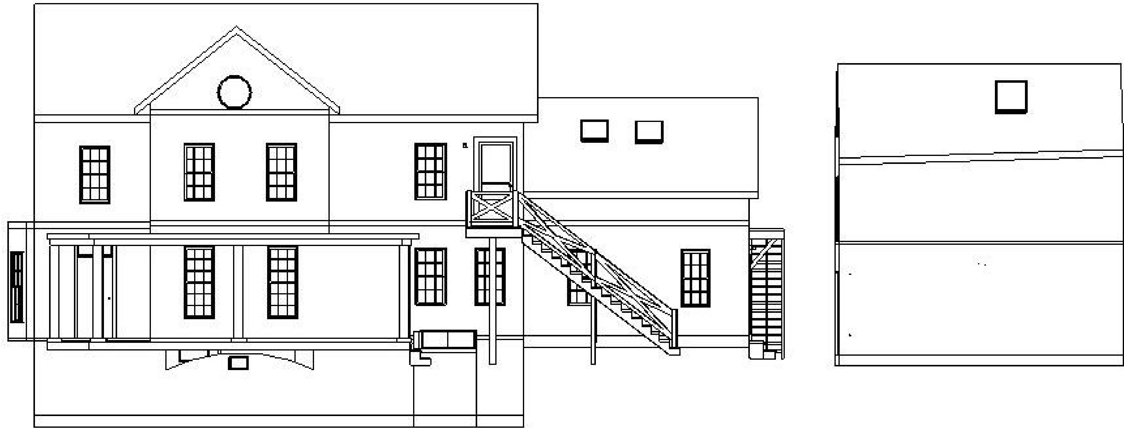
EXISTING NORTH ELEVATION
