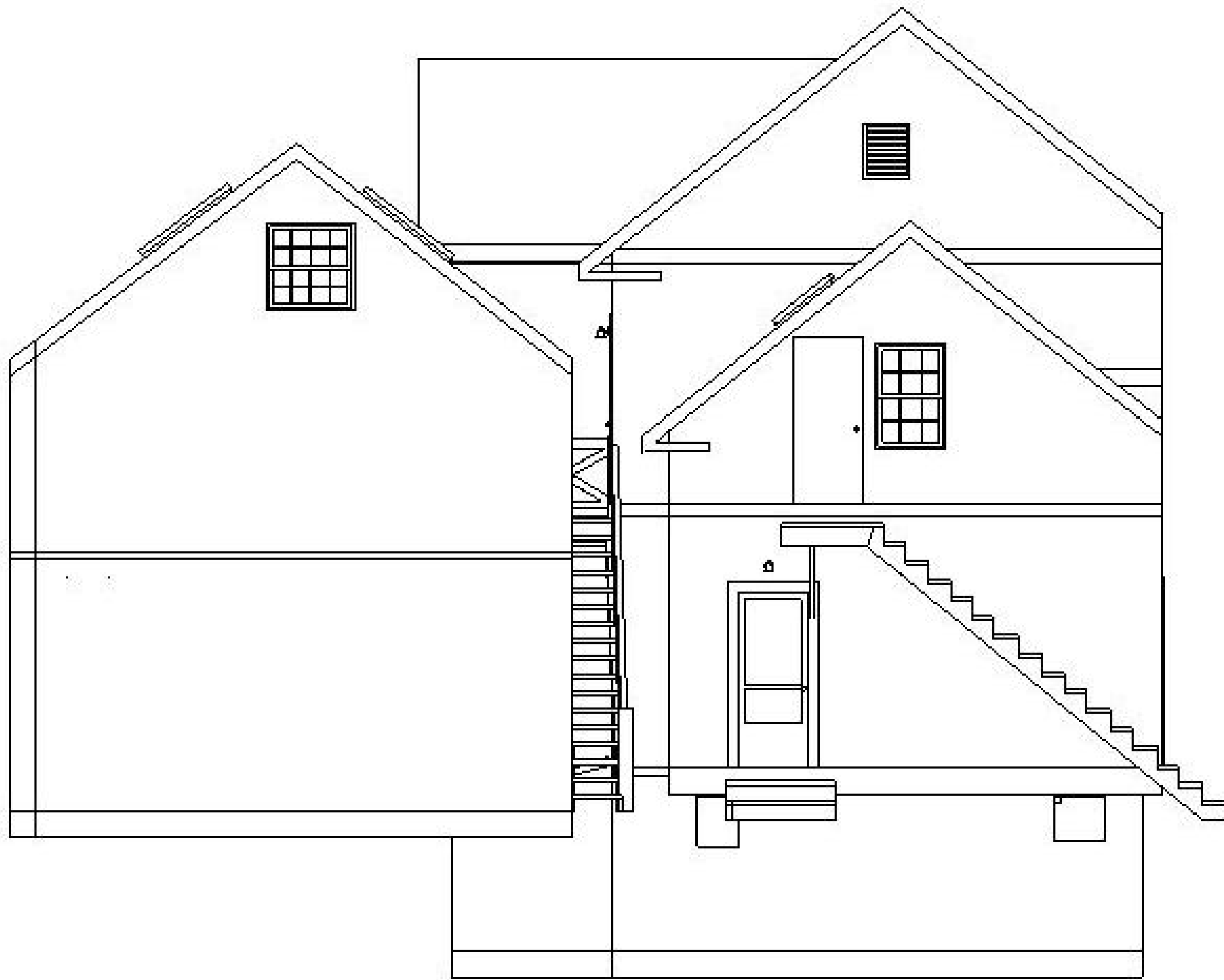
EXISTING WEST ELEVATION
