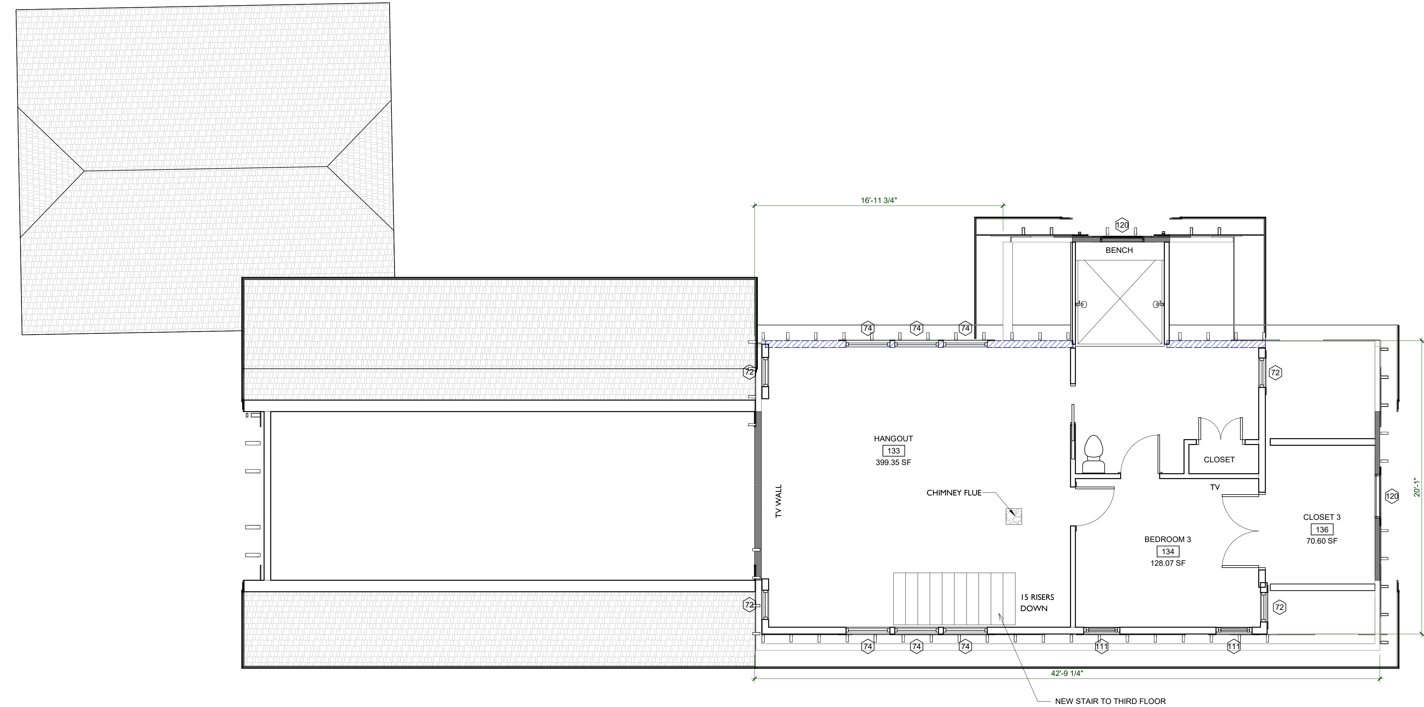
1 THIRD FLOOR PLAN 1/4" = 1'-0"
