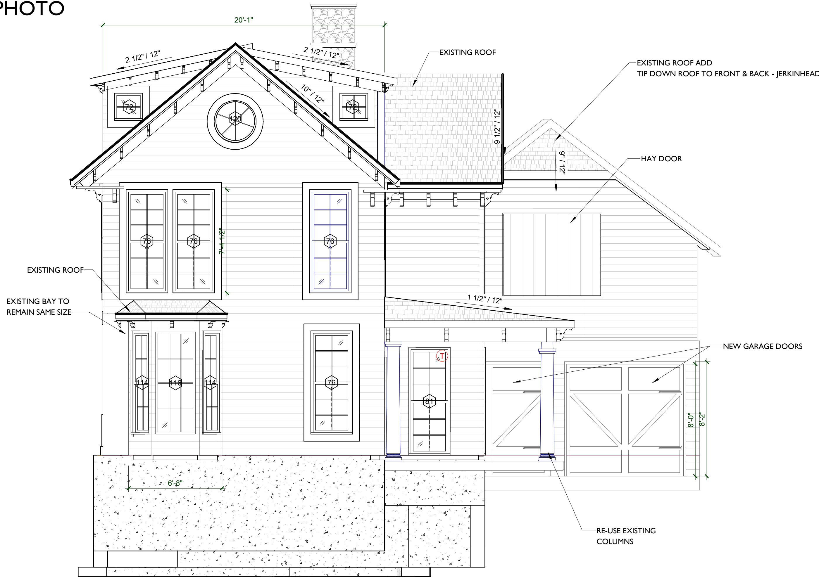
1 EAST ELEVATION 1/4" = 1'-0"
