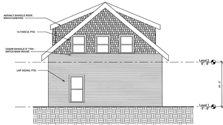
② Elevation 7 - a 1/4" = 1'-0"
