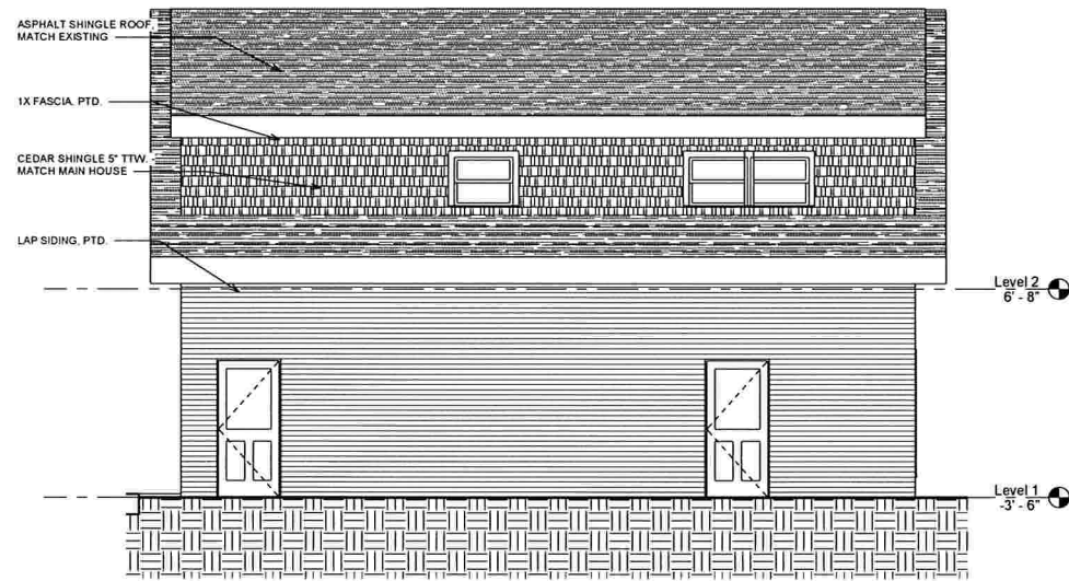
③ Elevation 6 - a 1/4" = 1'-0"
