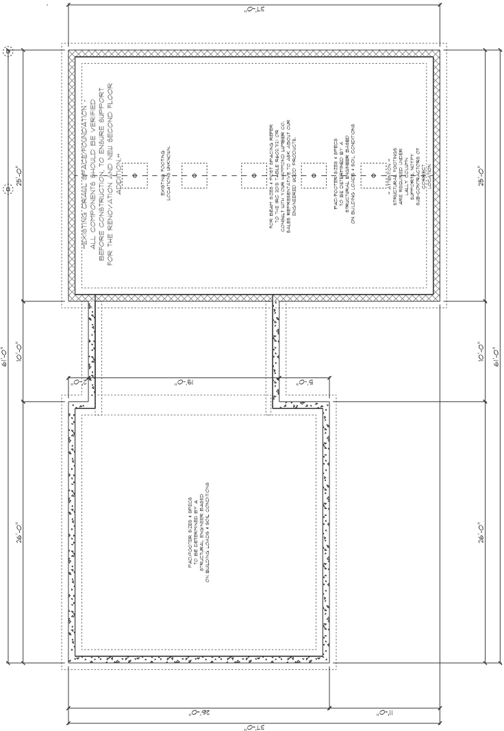
FOUNDATION SCALE: 1/4" = 1'-0"
