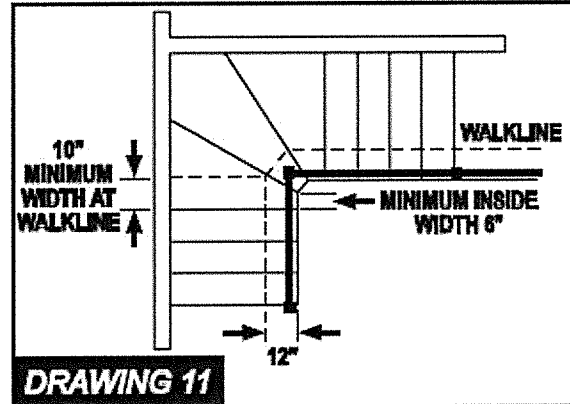
ALTERNATE WINDER TREAD DESIGNS
