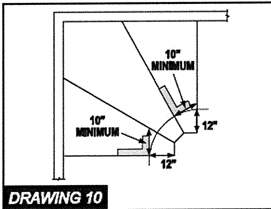
ALTERNATE WINDER TREAD DESIGNS
