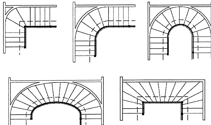
ALTERNATE WINDER TREAD DESIGNS
