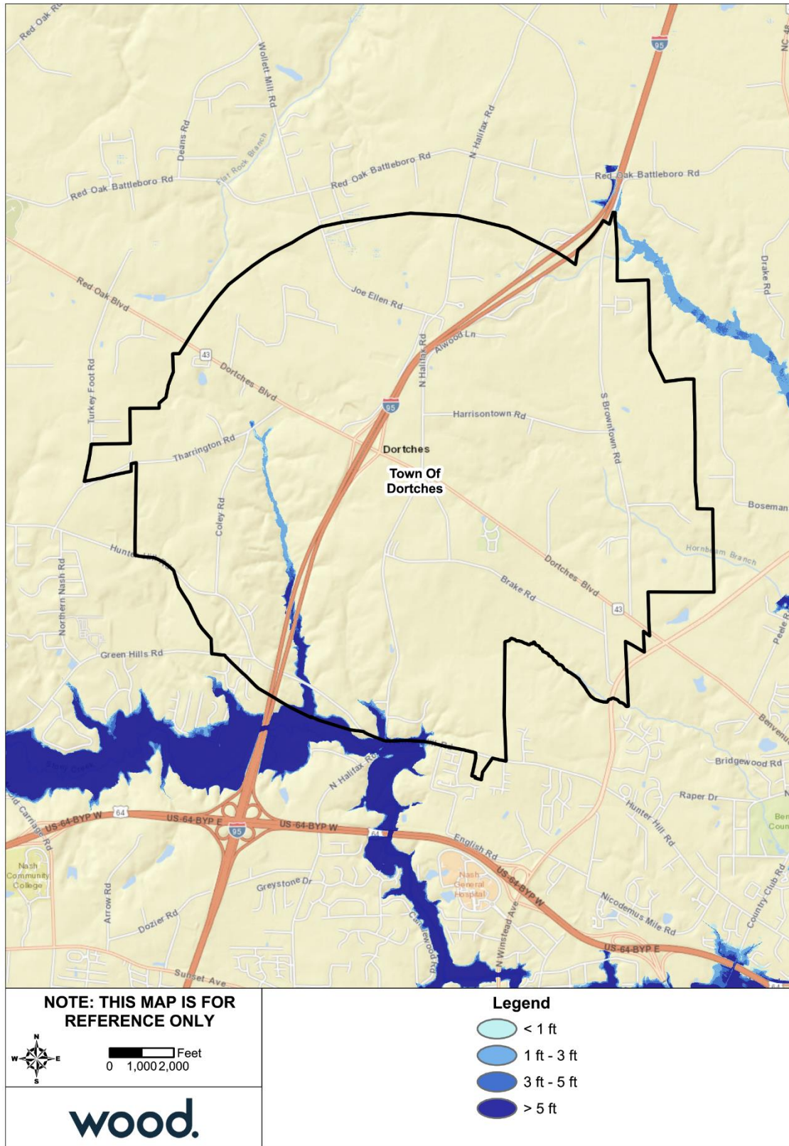
Figure J.3 – Flood Depth, 1%-Annual-Chance Floodplain, Town of Dortches
