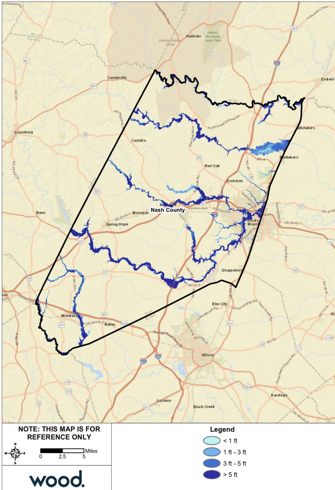
Figure 4.24 – Flood Depth, 100-Year Floodplain, Nash County
