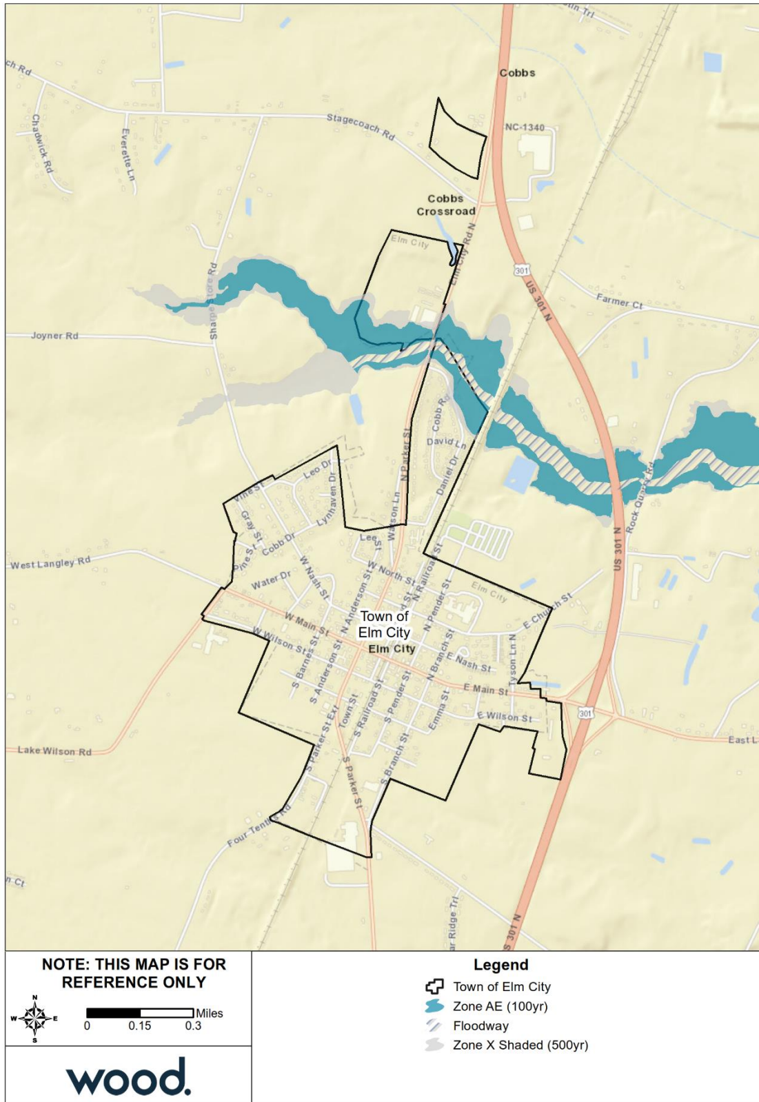
Figure K.2 – FEMA Flood Hazard Areas, Town of Elm City
