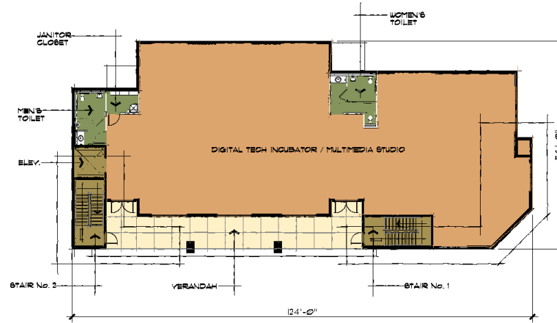
SCHEMATIC SOUTH BUILDING - SECOND FLOOR PLAN 3/32" = 1'-0"
