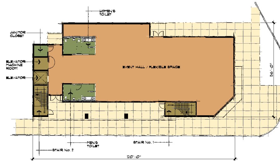
SCHEMATIC SOUTH BUILDING - FIRST FLOOR PLAN
