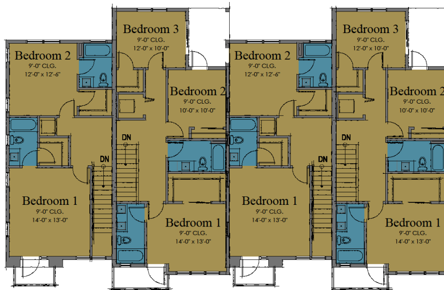
RESIDENTIAL - SCHEMATIC SECOND FLOOR PLAN
