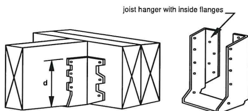
Figure 9 JOIST HANGERS
