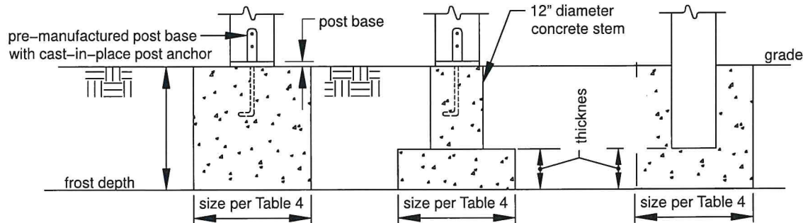
Figure 1 FOOTINGS
