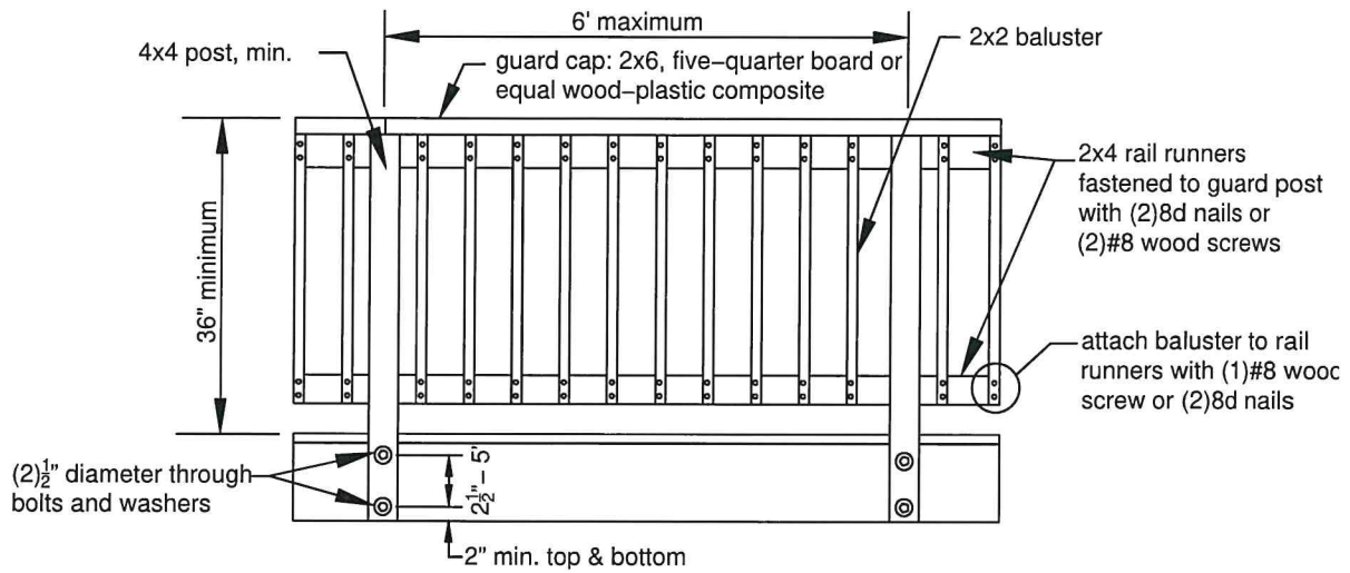
Figure 24 GUARDS
