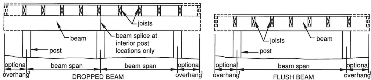
Figure 3 BEAM TYPES
