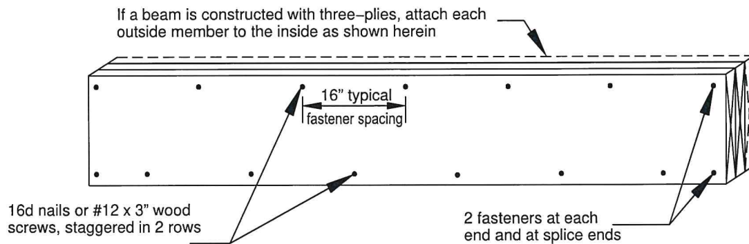
Figure 4 BEAM ASSEMBLY
