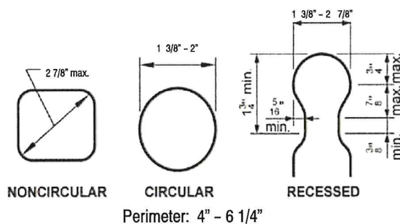
Figure 34 HANDRAIL GRASPABILITY
