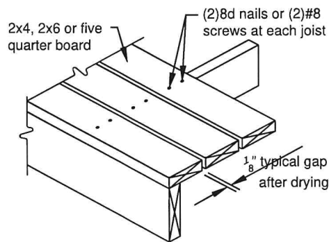
Figure 22 TYPICAL DECKING
