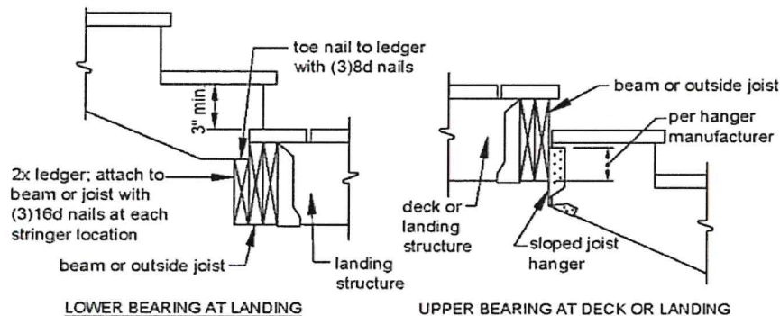
Figure 28 STRINGER BEARING
