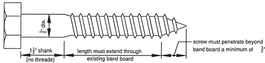
Figure 16 LAG SCREW
