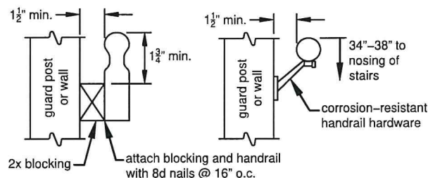
Figure 34 HANDRAIL GRASPABILITY
