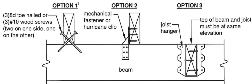
Figure 8 JOIST-TO-BEAM CONNECTIONS
