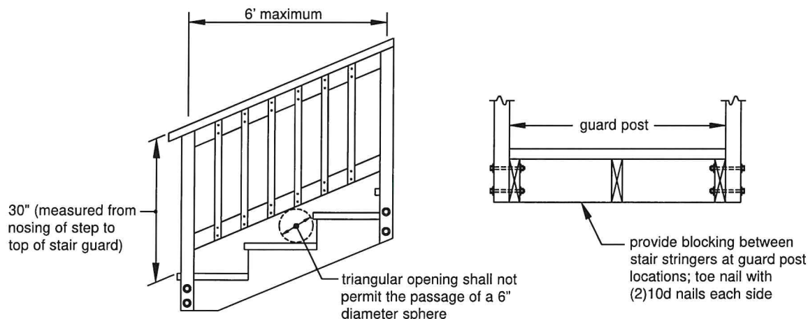
Figure 32 STAIR GUARDS
