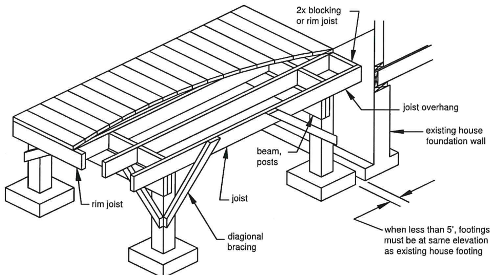
Figure 17 FREE-STANDING DECK
