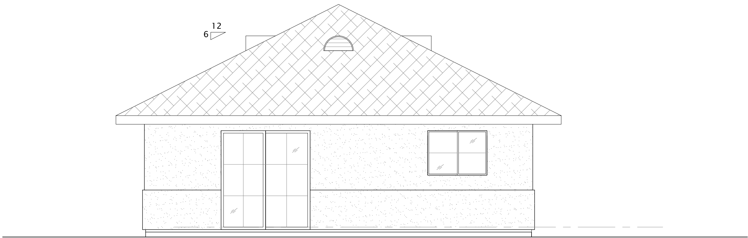
B LEFT SIDE ELEVATION - WILLOW SCALE: 1/4" = 1'-0"
