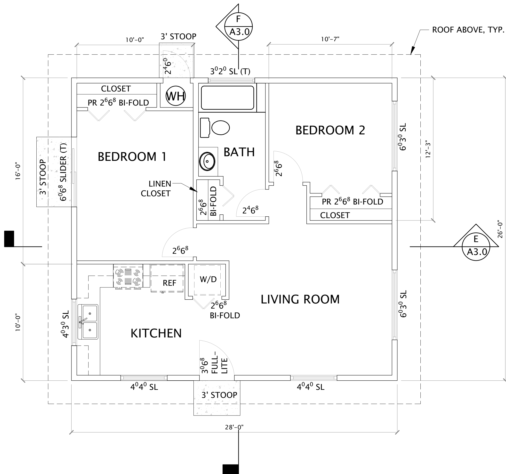
1 FLOOR PLAN— 728 SQ. FT. SCALE: 1/4" = 1'-0"
