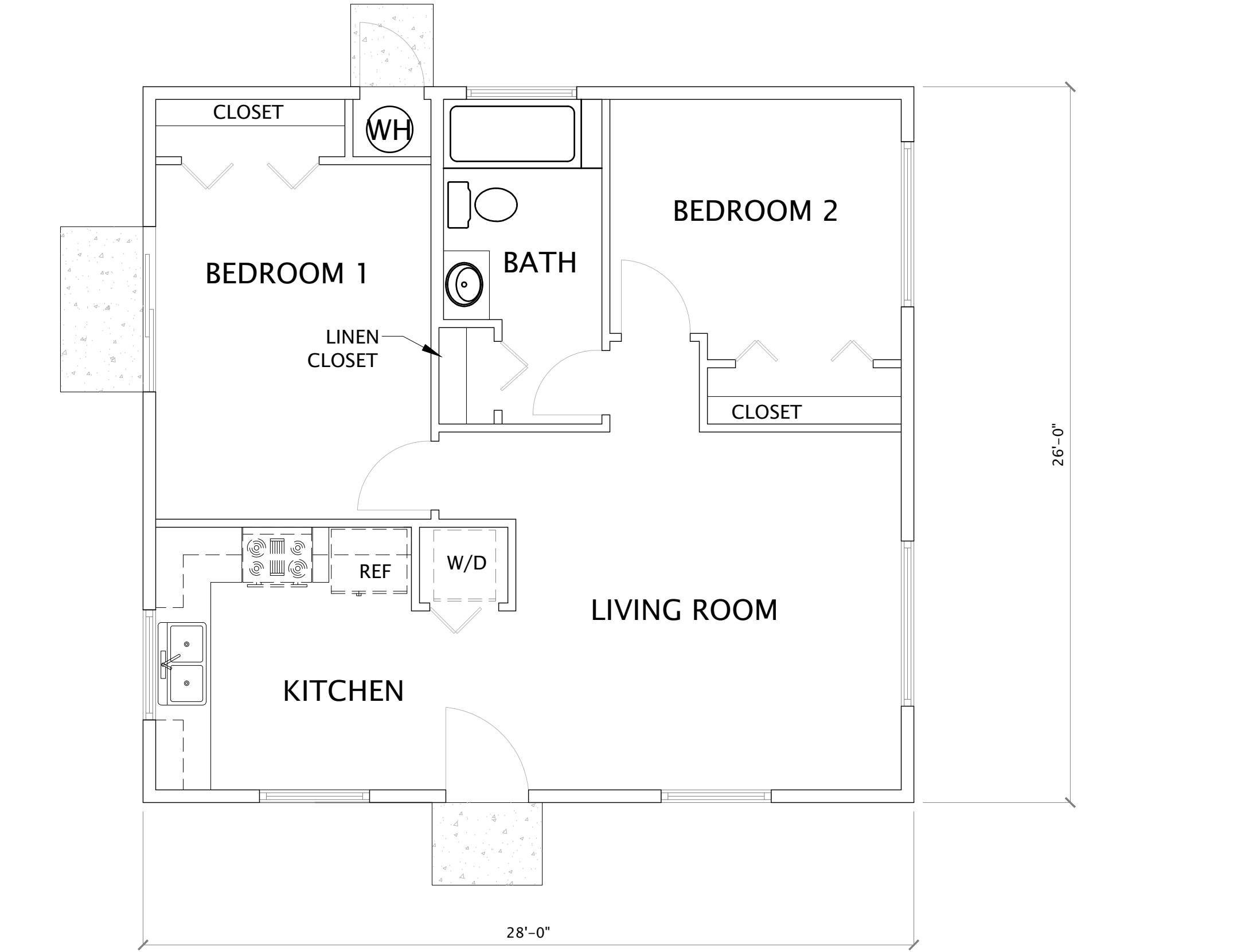
1 FLOOR PLAN— 728 SQ. FT. SCALE: 1/4" = 1'-0"
