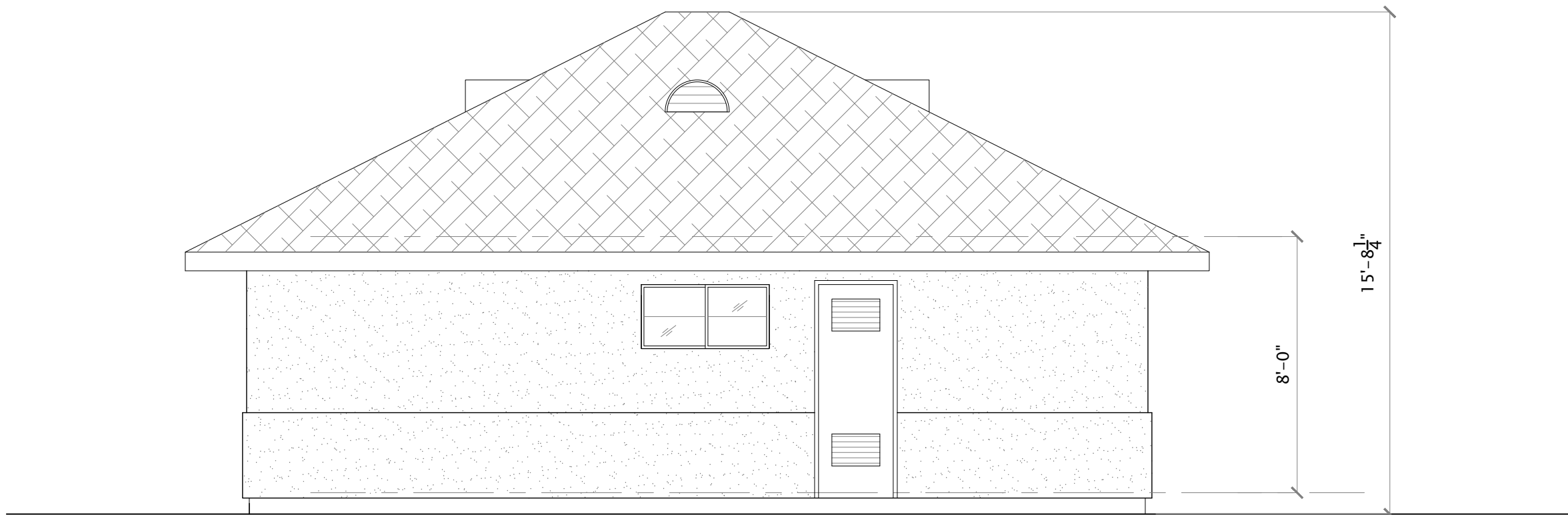
D REAR ELEVATION - WILLOW SCALE: 1/4" = 1'-0"
