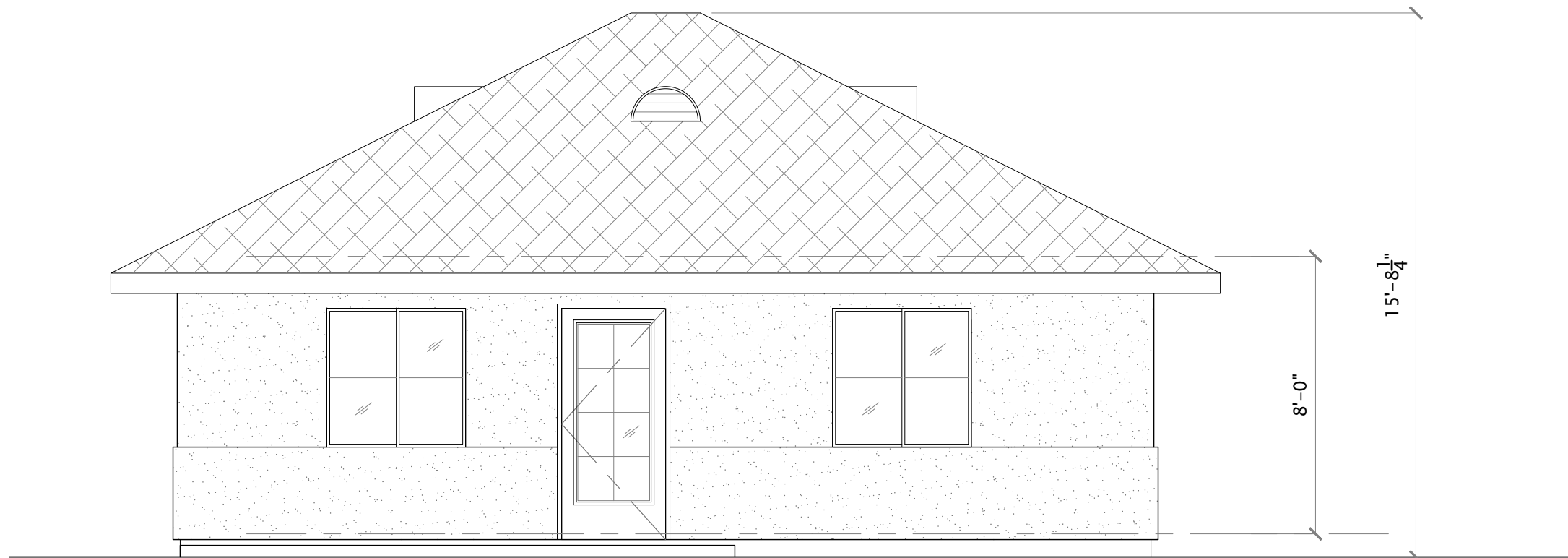
A FRONT ELEVATION - WILLOW SCALE: 1/4" = 1'-0"
