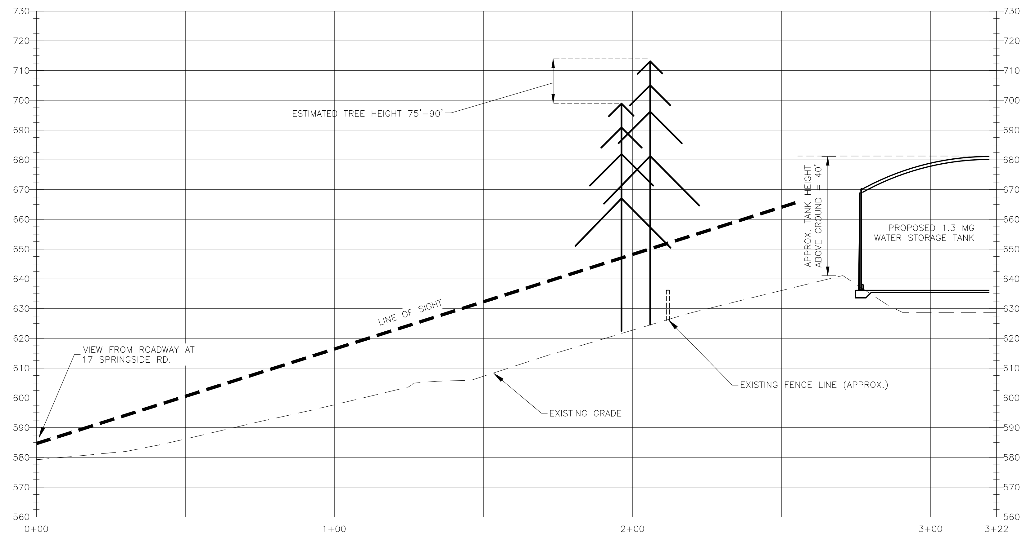
LINE OF SIGHT PROFILE VIEW SCALE: H- 1" = 20' V- 1" = 20'
