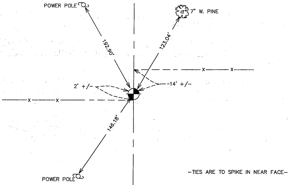
SKETCH OF REFERENCE TIES FROM TIE SHEET 939
