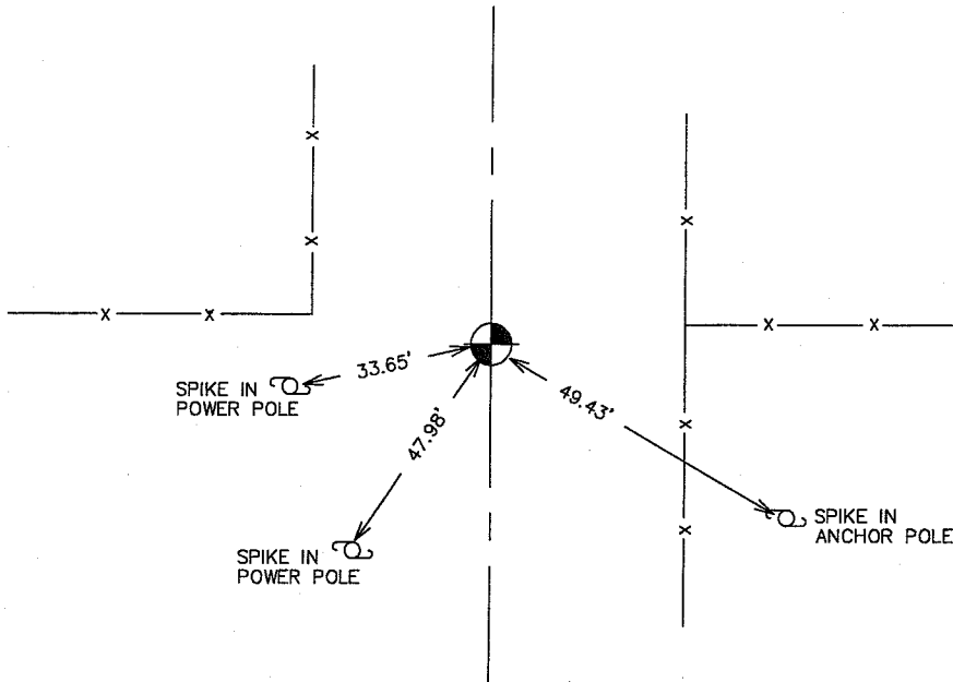
SKETCH OF REFERENCE TIES FROM TIE SHEET 939
