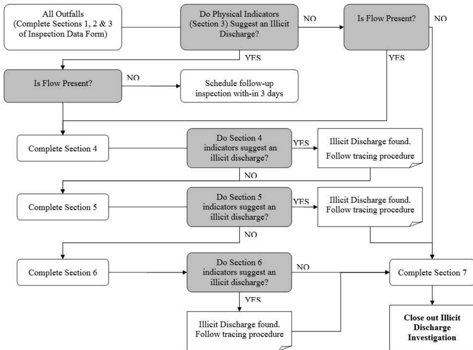
Figure 12: Outfall Inspection Procedure Flow Chart
