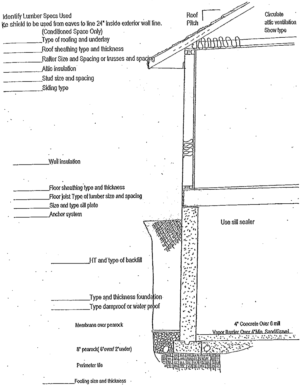
Sample Construction Detail – Heated Space — Residential Addition
