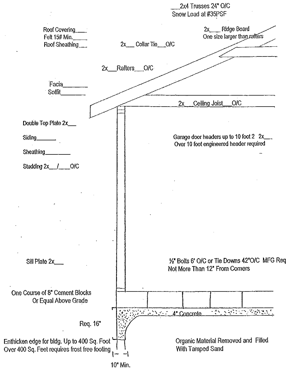
Sample Detached Garage Construction Detail — Show pitch of roof and wall height
