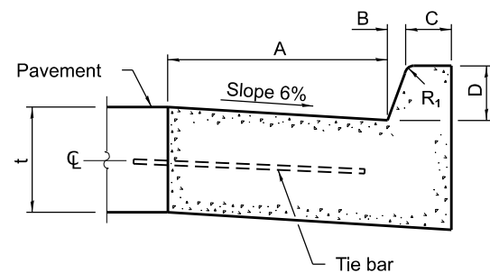
BARRIER CURB
