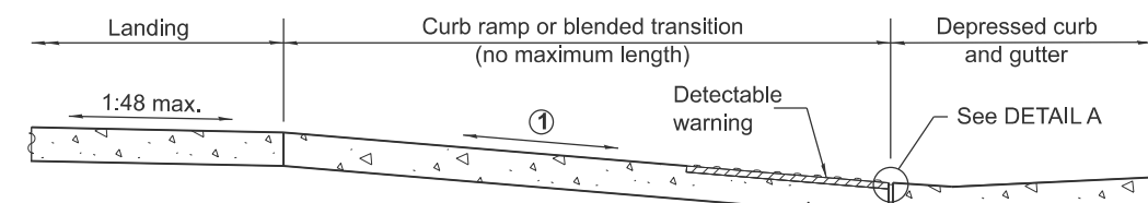
SECTION B-B
