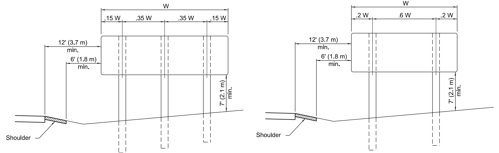
POST SPACING FOR NON-FREEWAY SIGN PANELS
