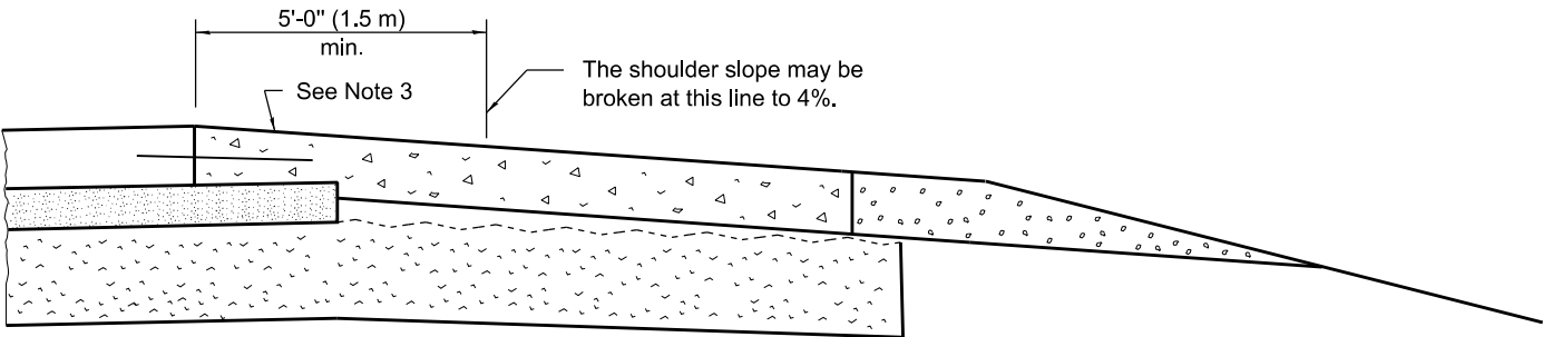
SHOULDER FOR SUPERELEVATED PAVEMENT (Outside of curve)
