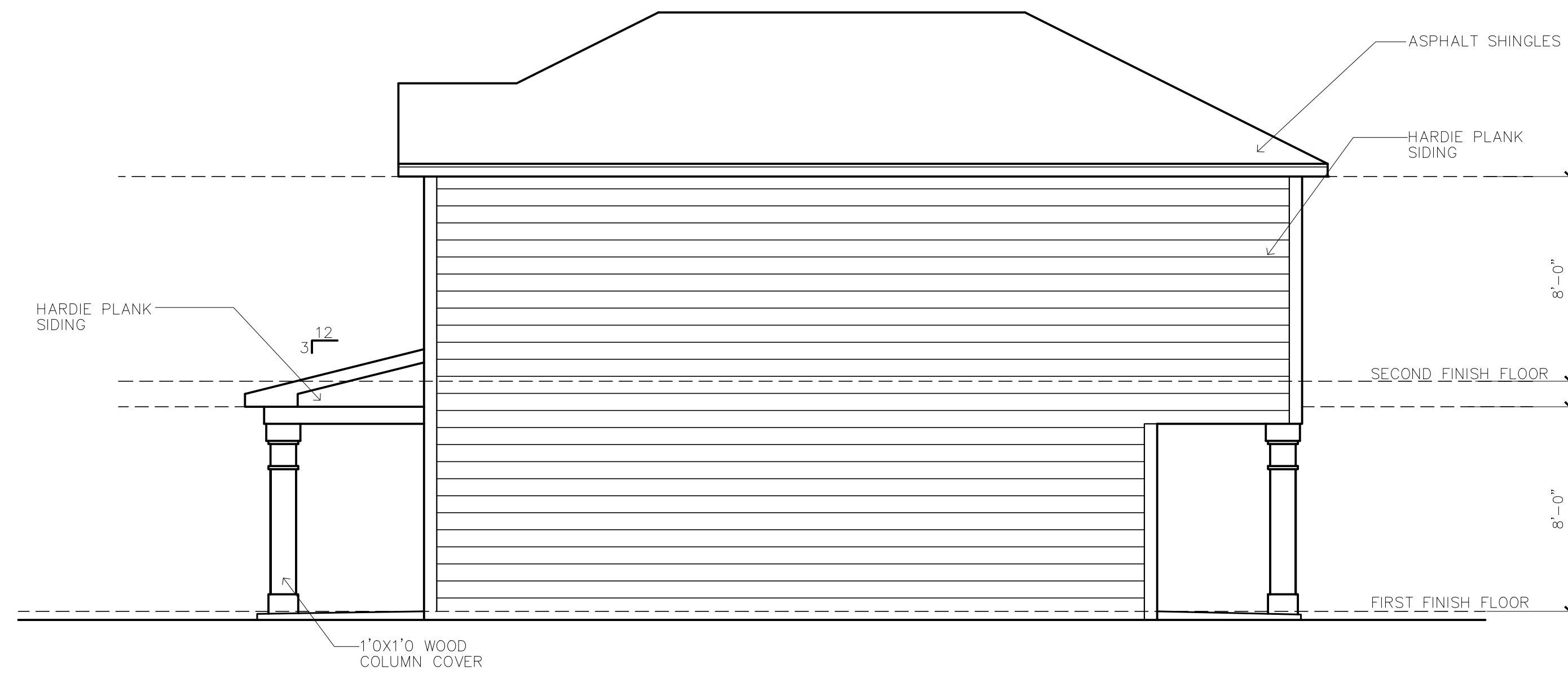
2 RIGHT ELEVATION SCALE 1/4"=1'-0"
