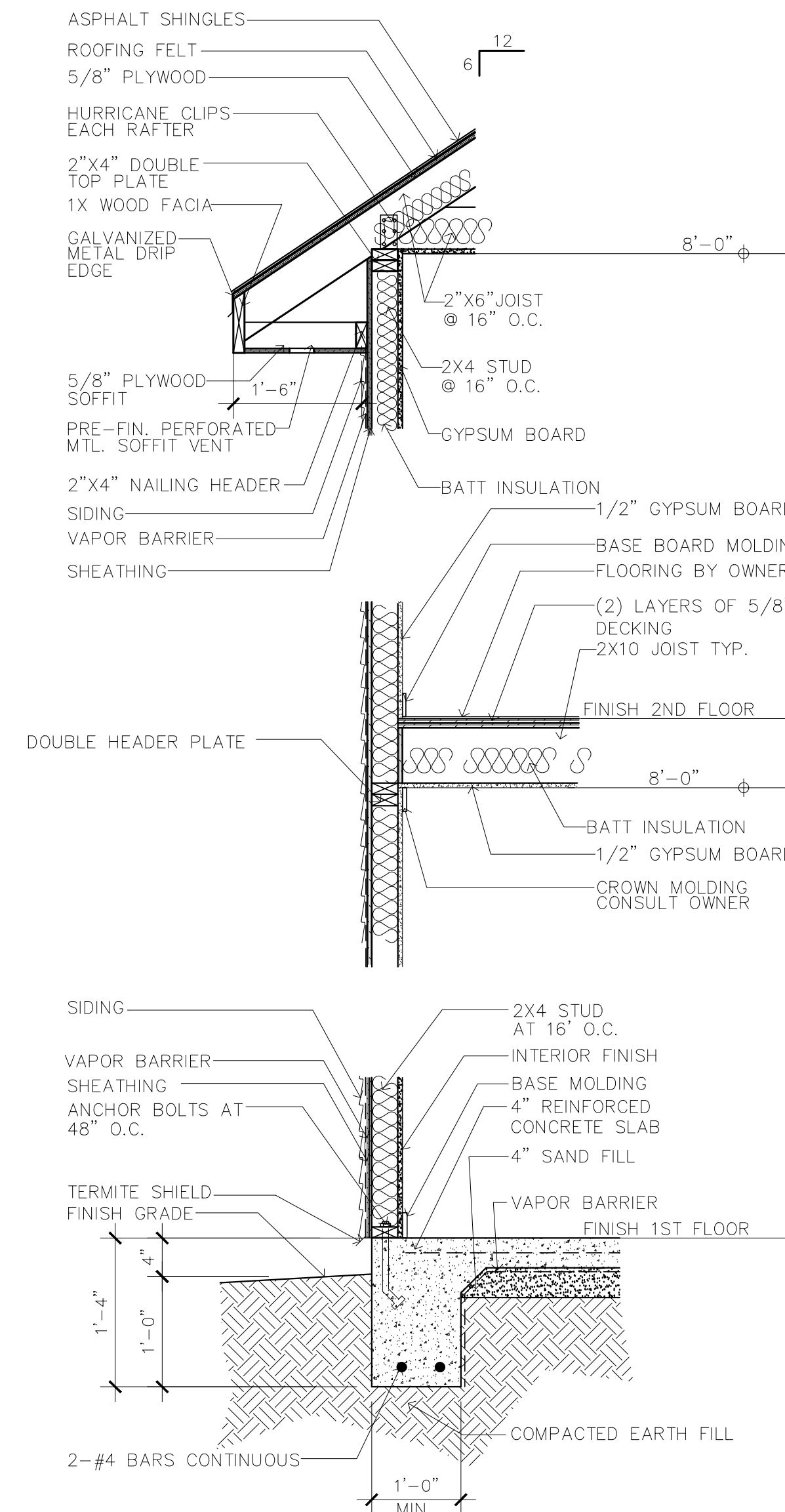
3 DETAIL 1 NTS
