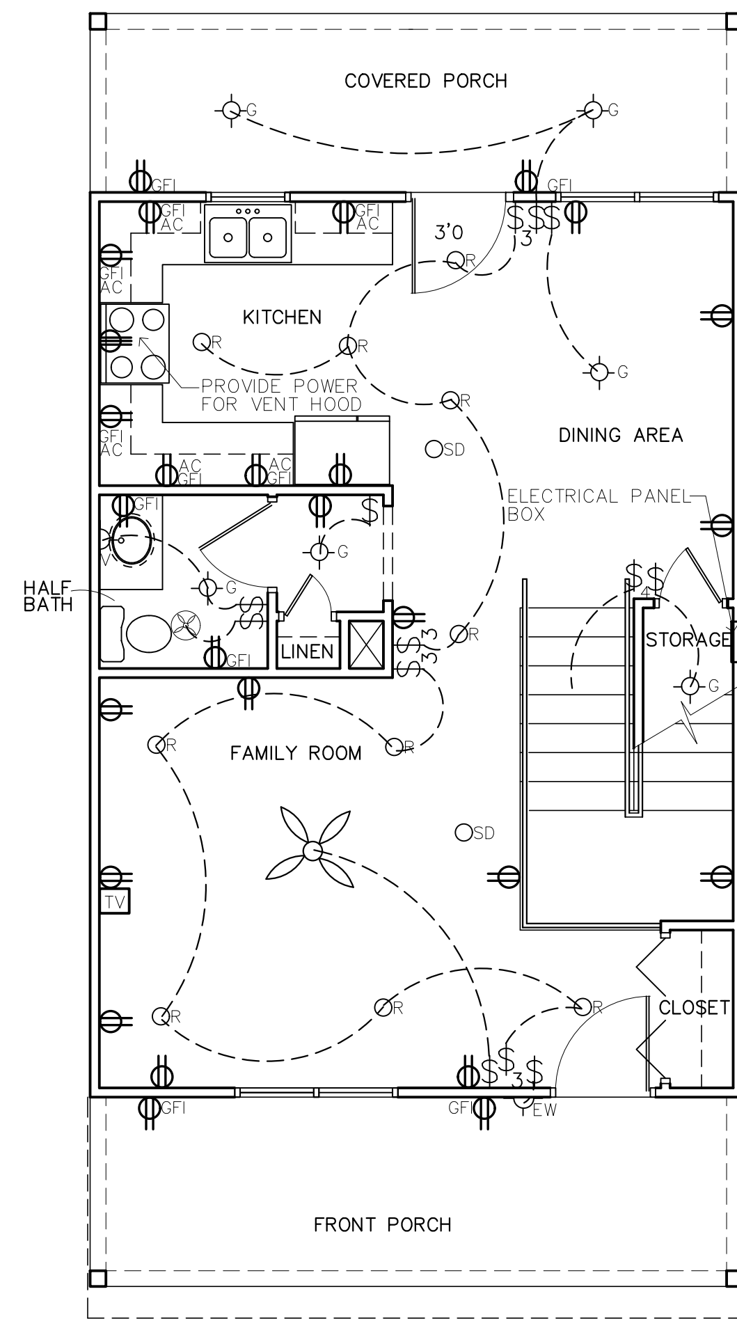
1 ELECTRICAL PLAN FIRST FLOOR SCALE 1/4"=1'-0"
