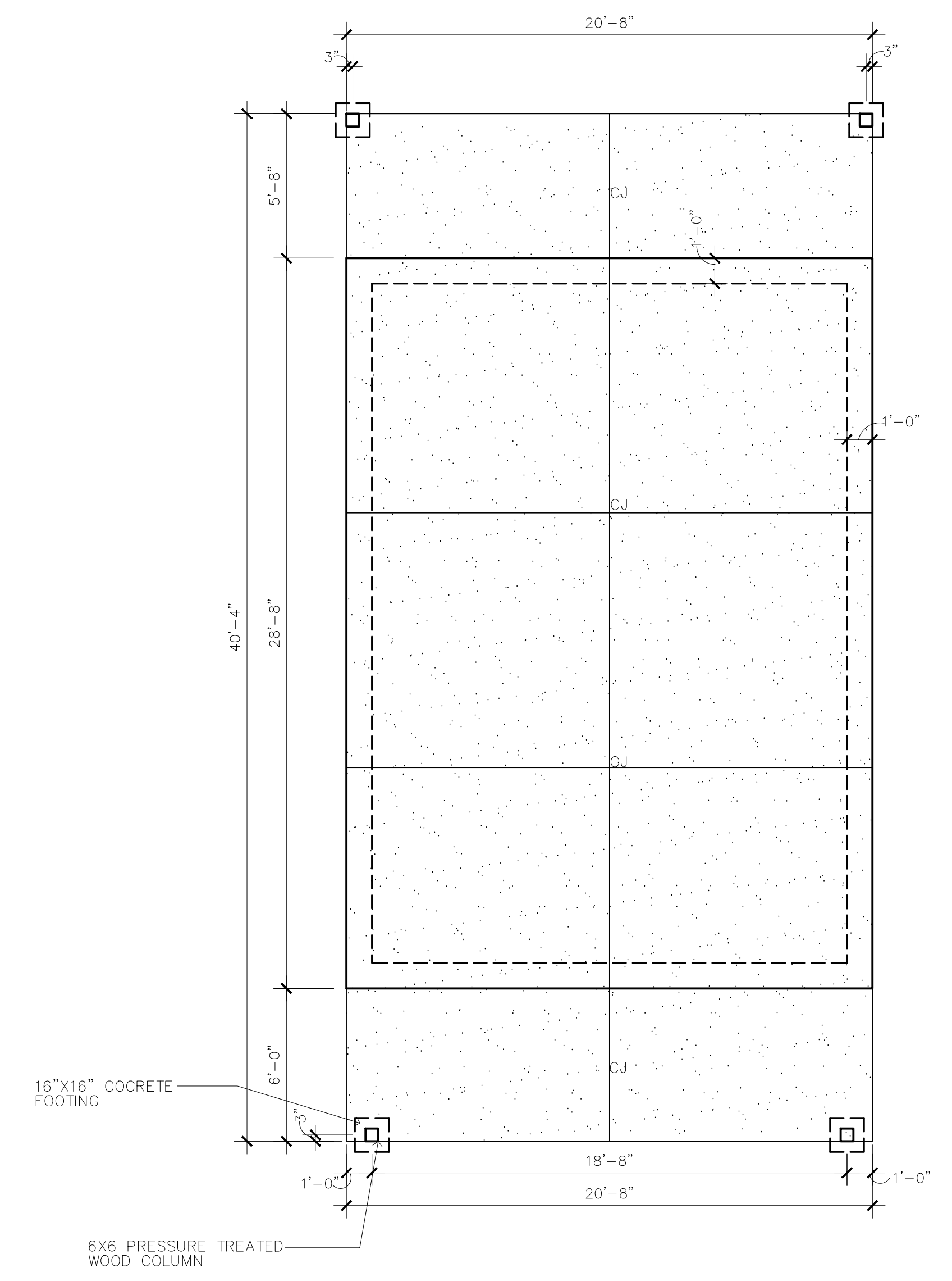
3 A3.0 FOUNDATION PLAN SCALE 1/4"=1'-0"
