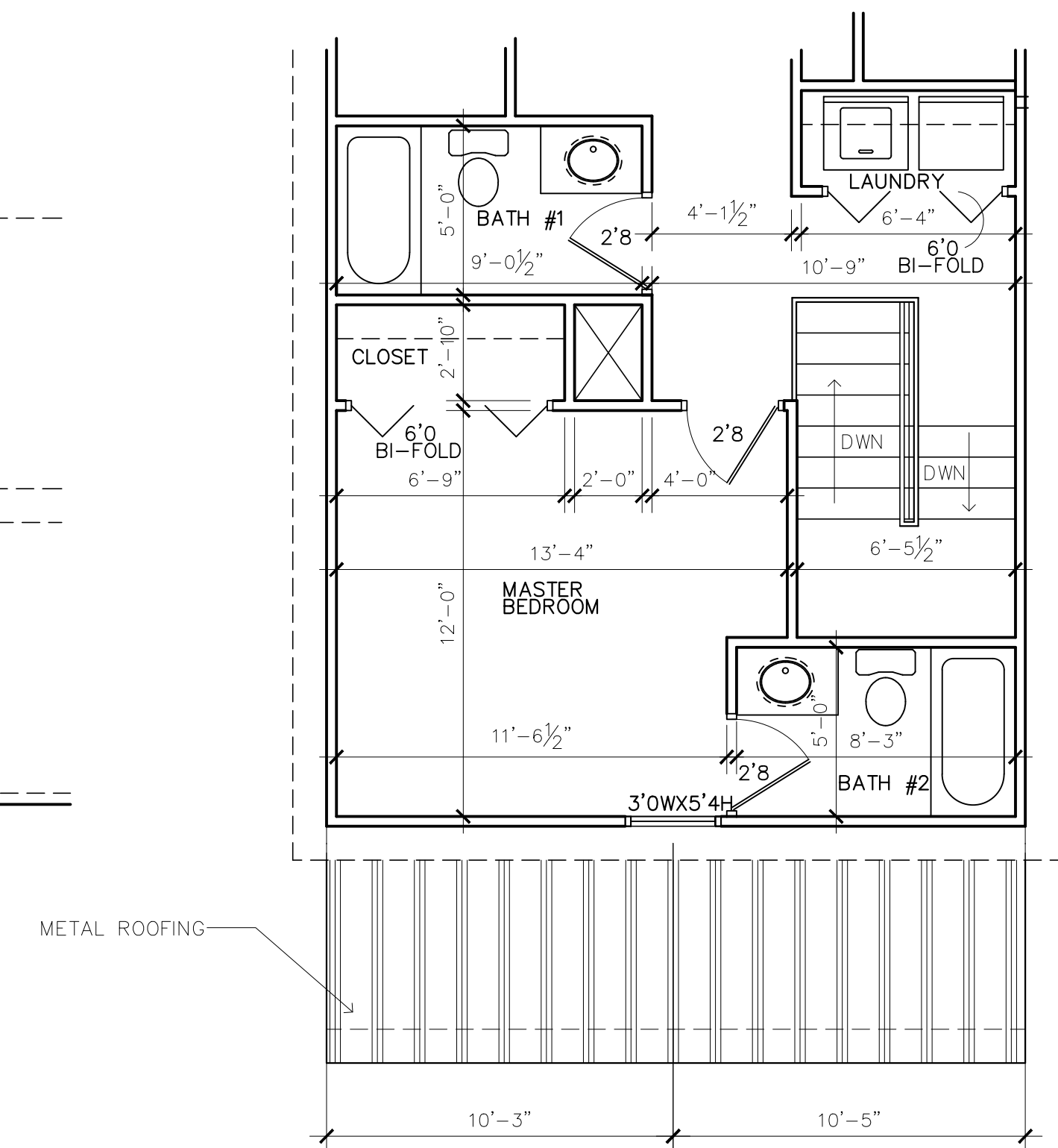
4A PARTIAL SECOND FLOOR PLAN SCALE 1/4"=1'-0"
