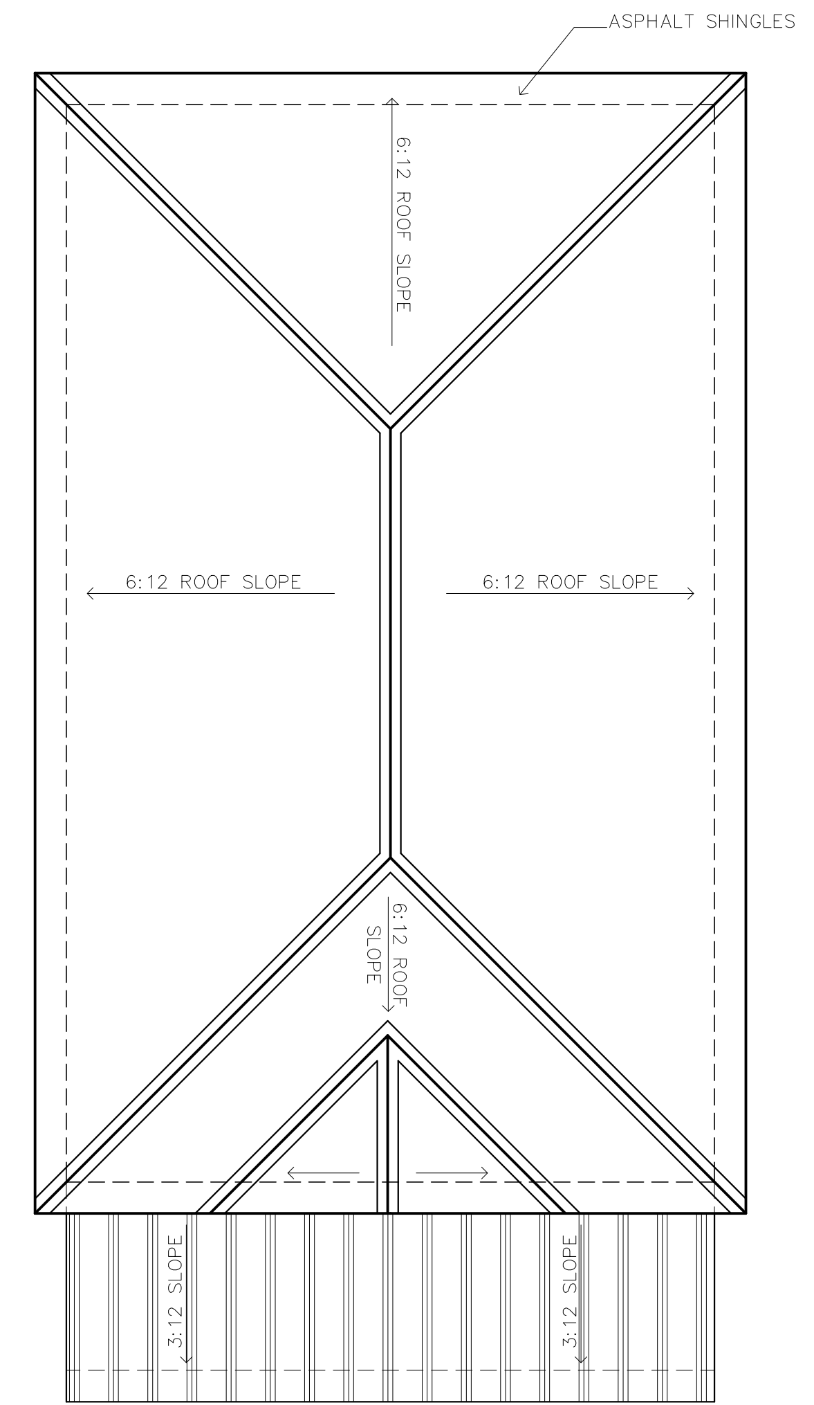
2A ROOF PLAN SCALE 1/4"=1'-0"
