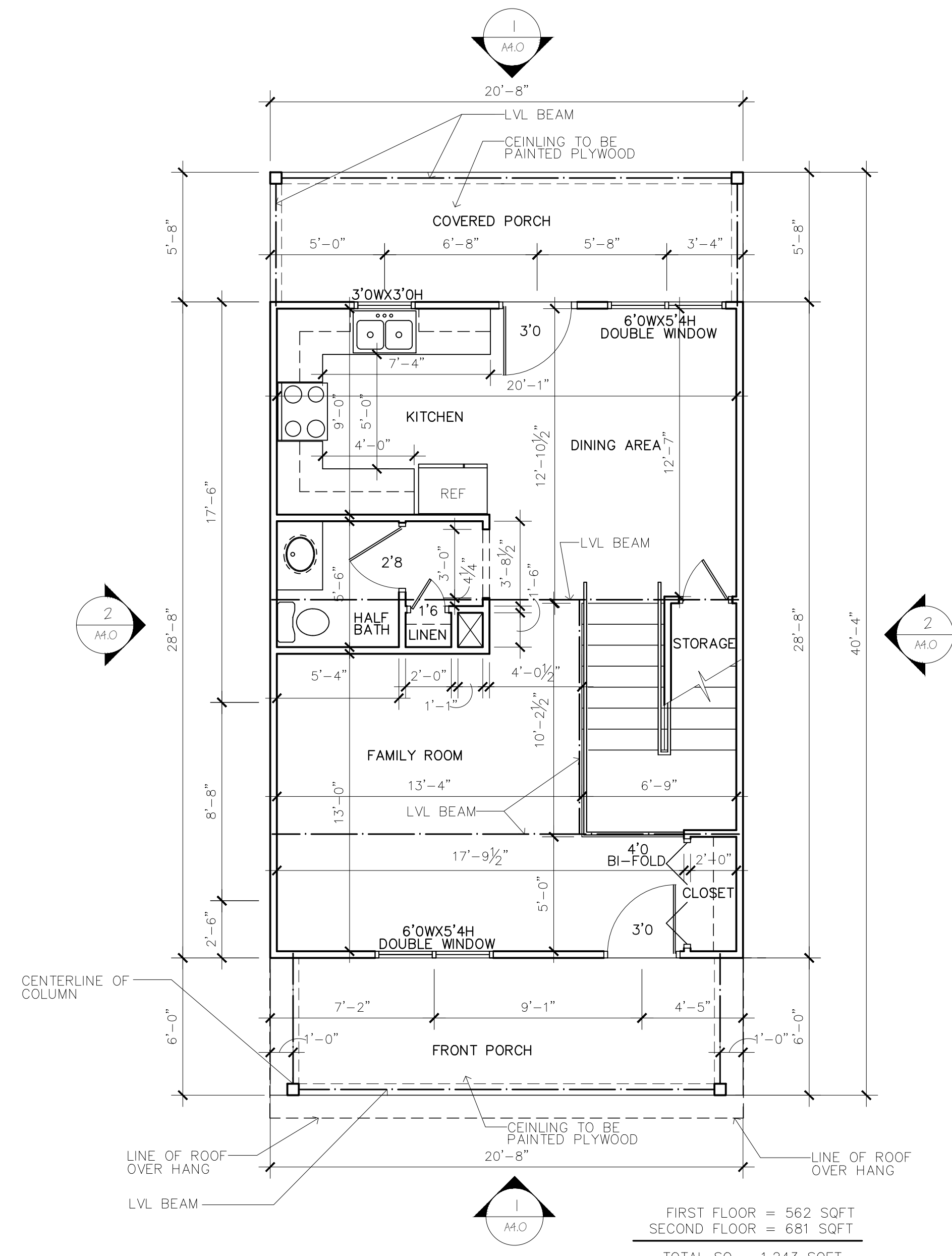
1 A3.0 FIRST FLOOR PLAN SCALE 1/4"=1'-0"
