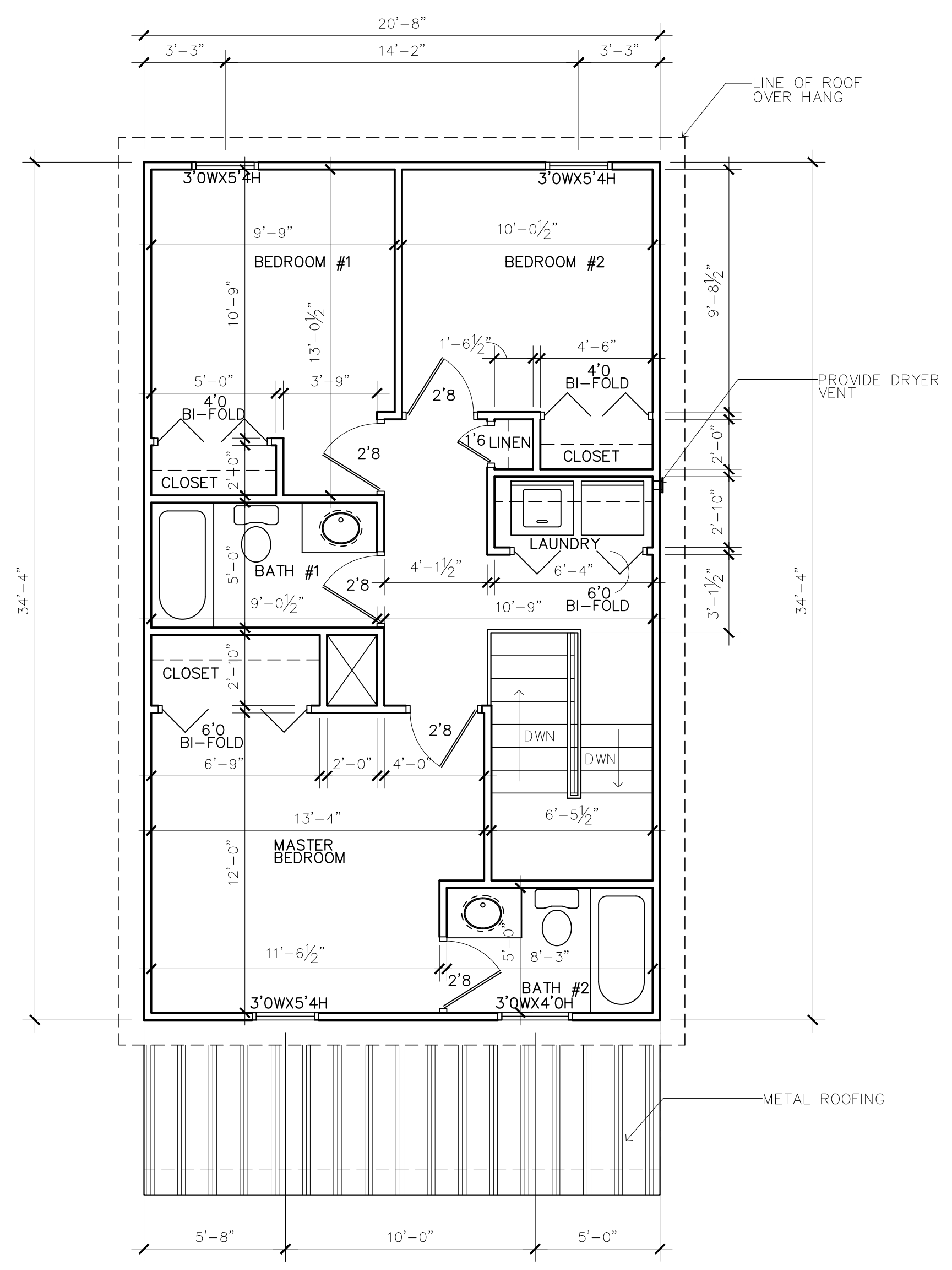
2 A3.0 SECOND FLOOR PLAN SCALE 1/4"=1'-0"
