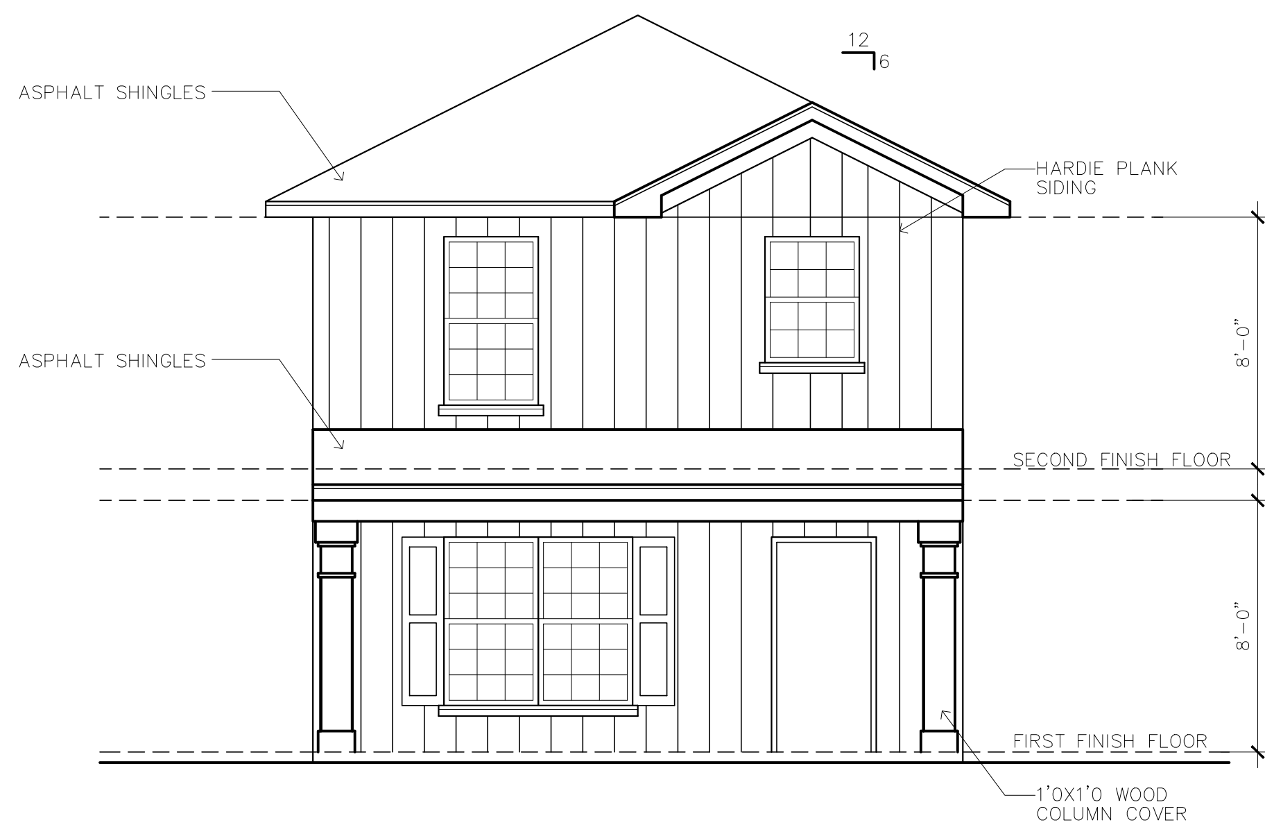
1 FRONT ELEVATION SCALE 1/4"=1'-0"
