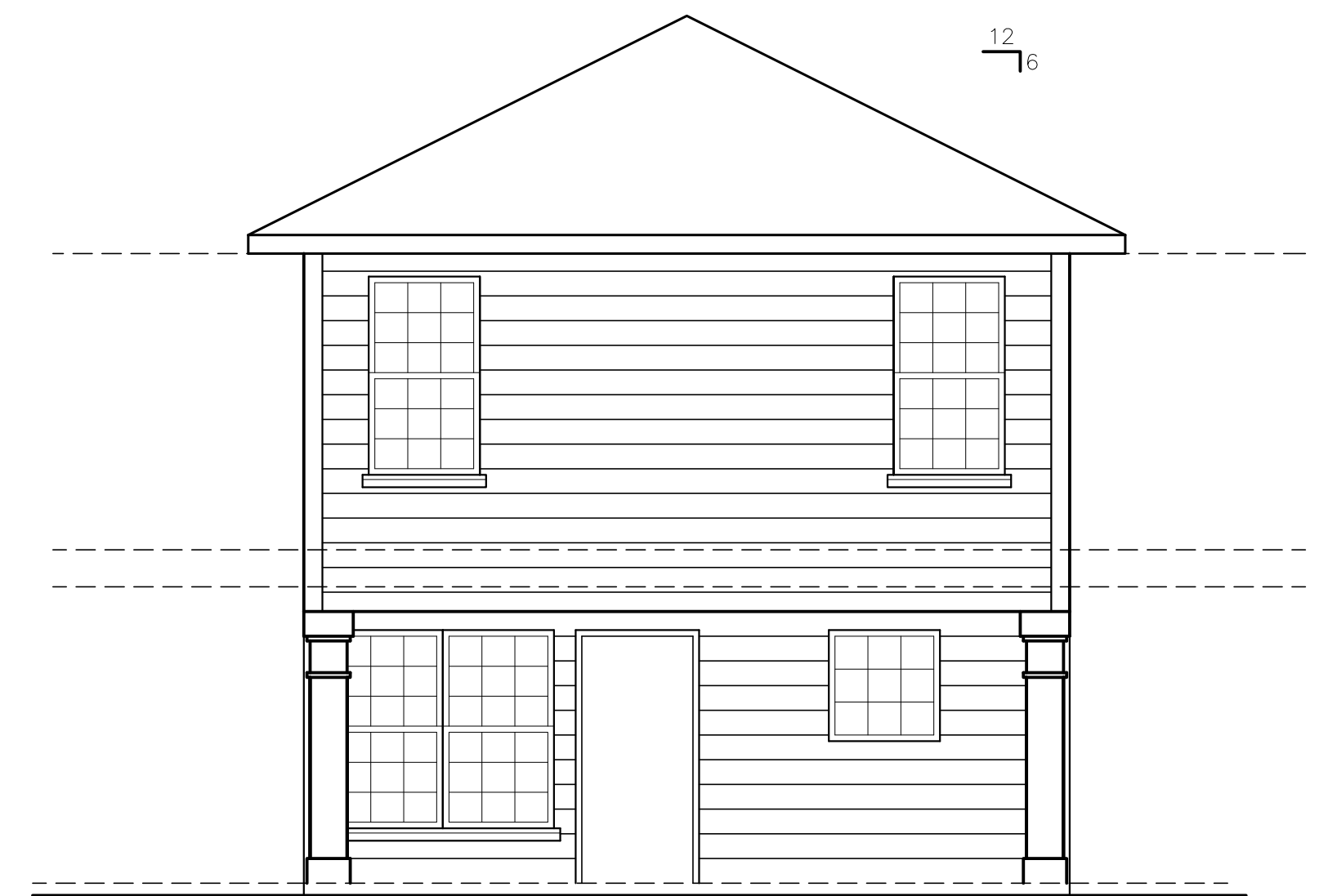
3 REAR ELEVATION SCALE 1/4"=1'-0"
