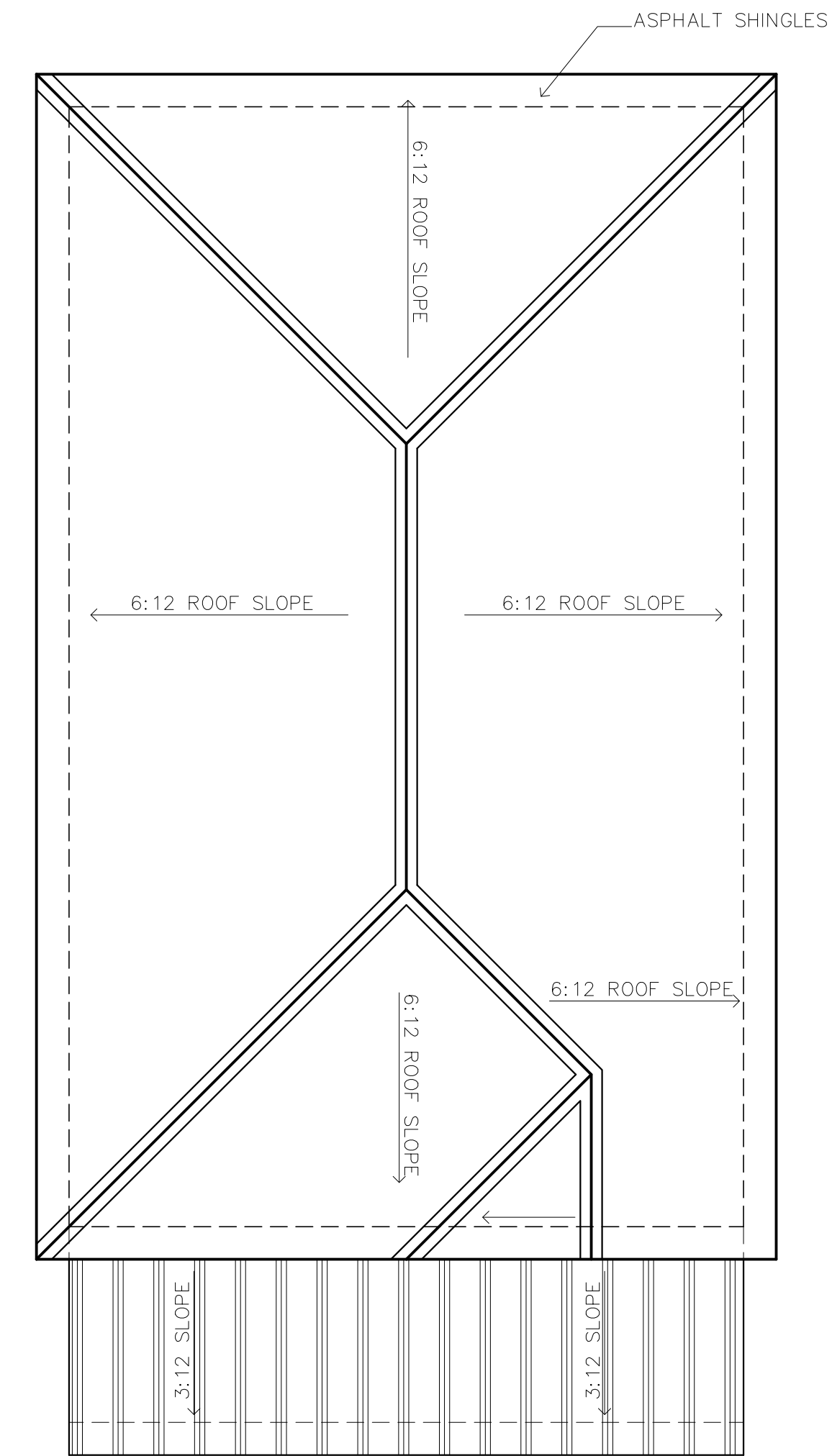
4 ROOF PLAN SCALE 1/4"=1'-0"
