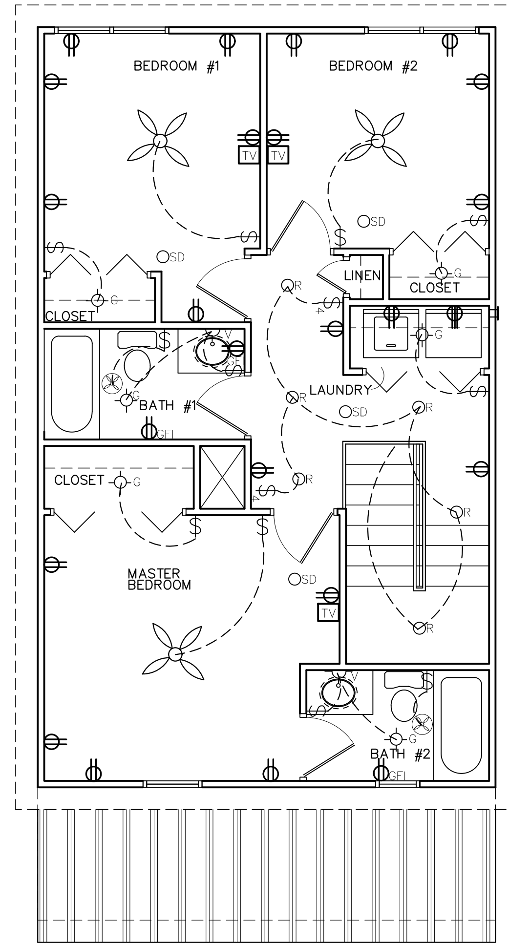
2 ELECTRICAL PLAN SECOND FLOOR SCALE 1/4"=1'-0"
