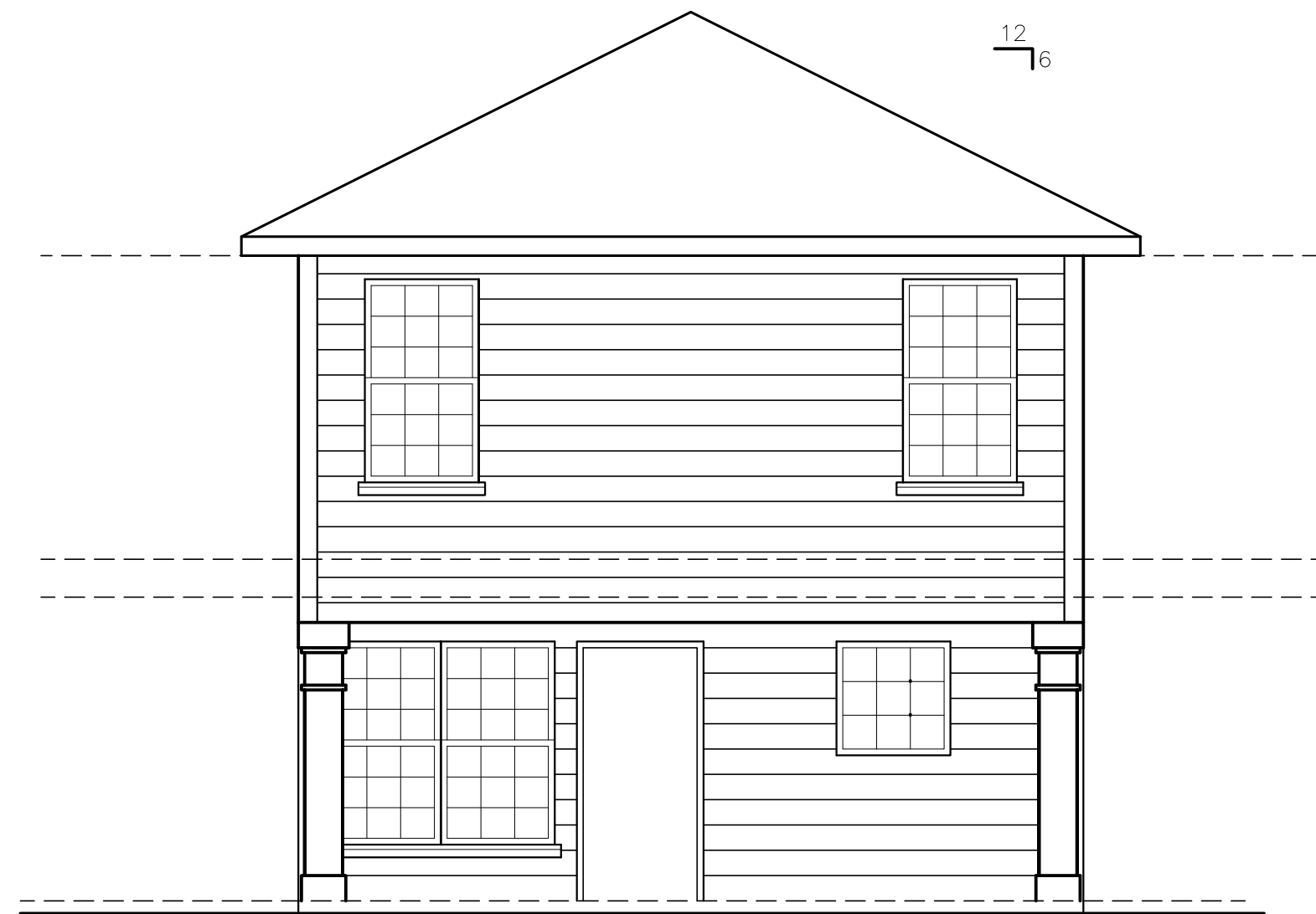
3 REAR ELEVATION SCALE 1/4"=1'-0"
