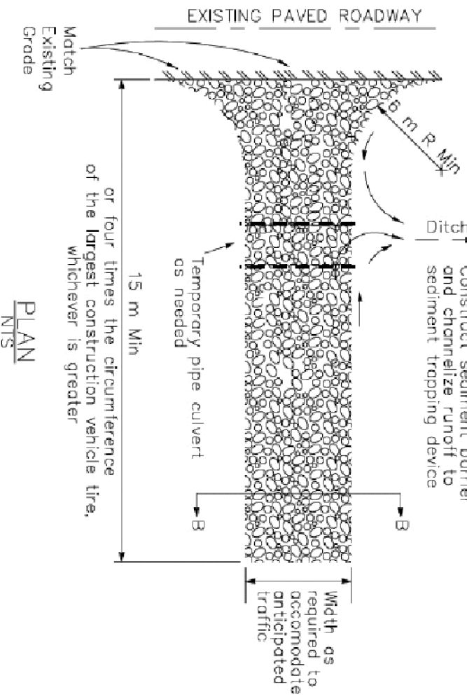
Stabilized Construction Entrance/Exit (Type 1)
