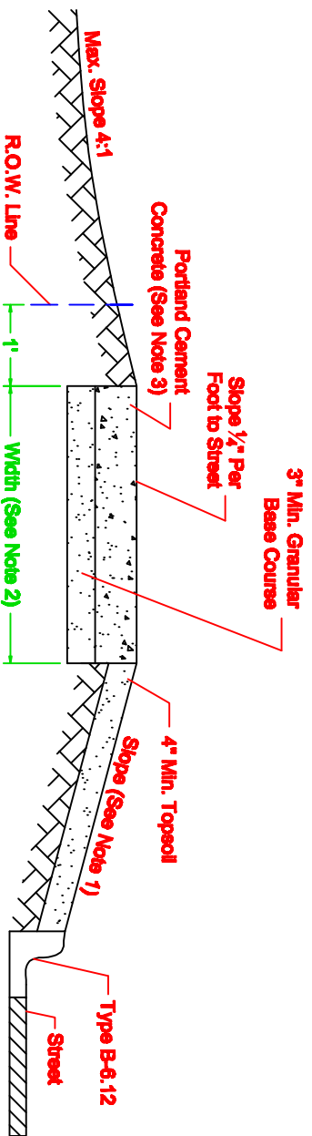
Typical Sidewalk Section in Filled Area
