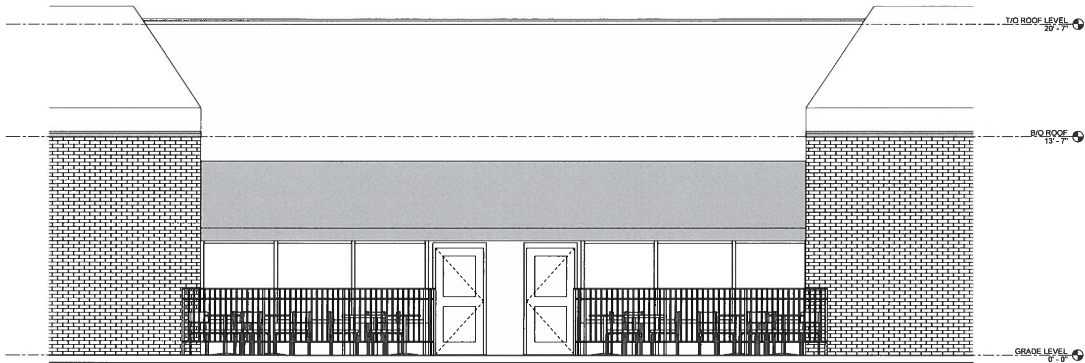
② FRONT ELEVATION 3/8" = 1'-0"
