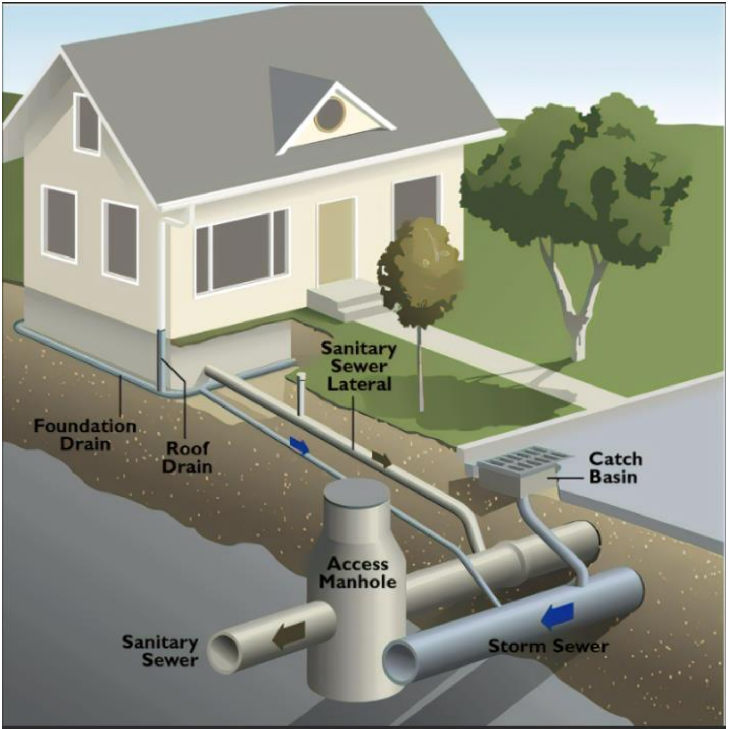
TYPICAL HOUSE SANITARY AND STORM SEWER LATERAL DIAGRAM
