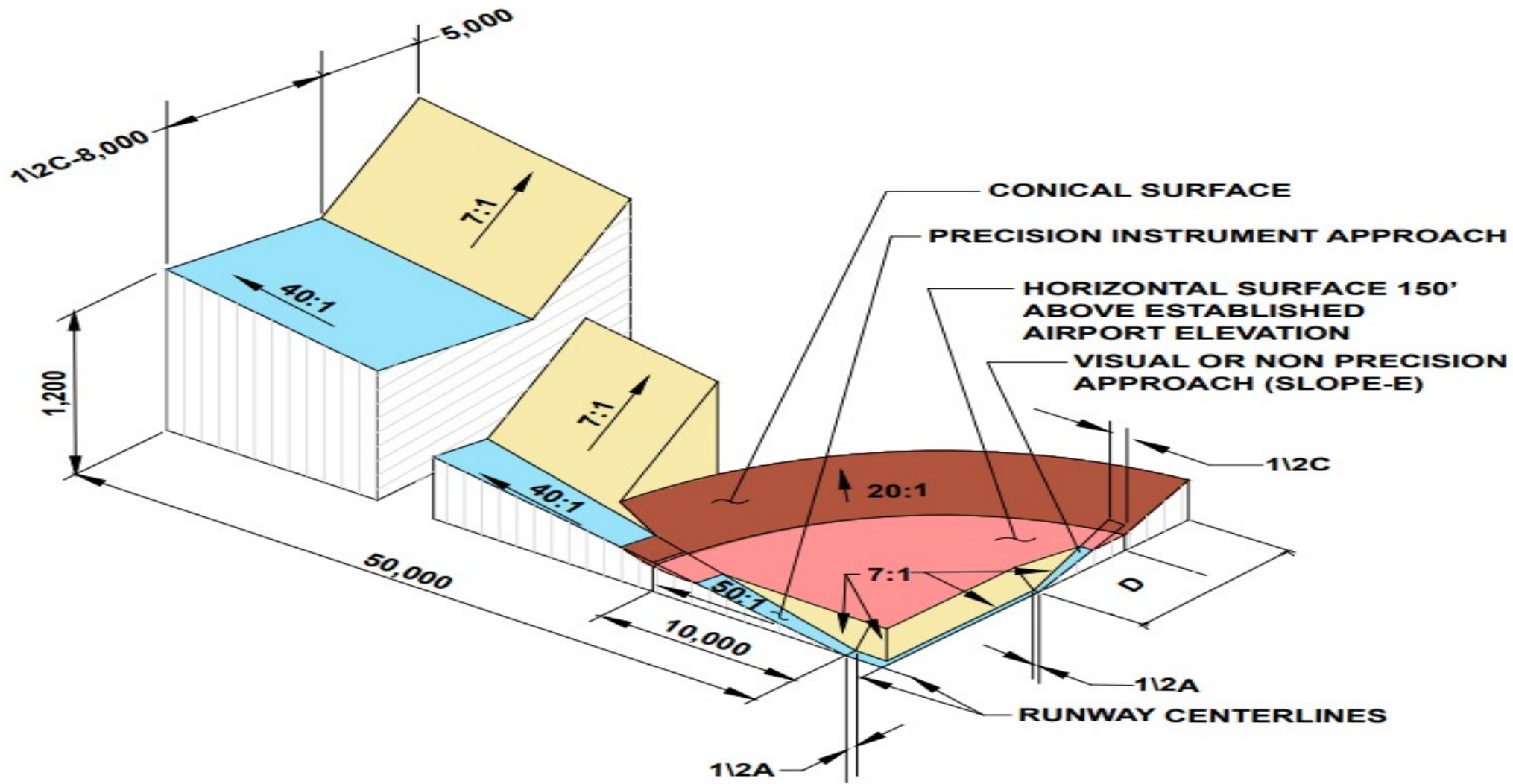
14 CFR Part 77 Imaginary Surfaces
